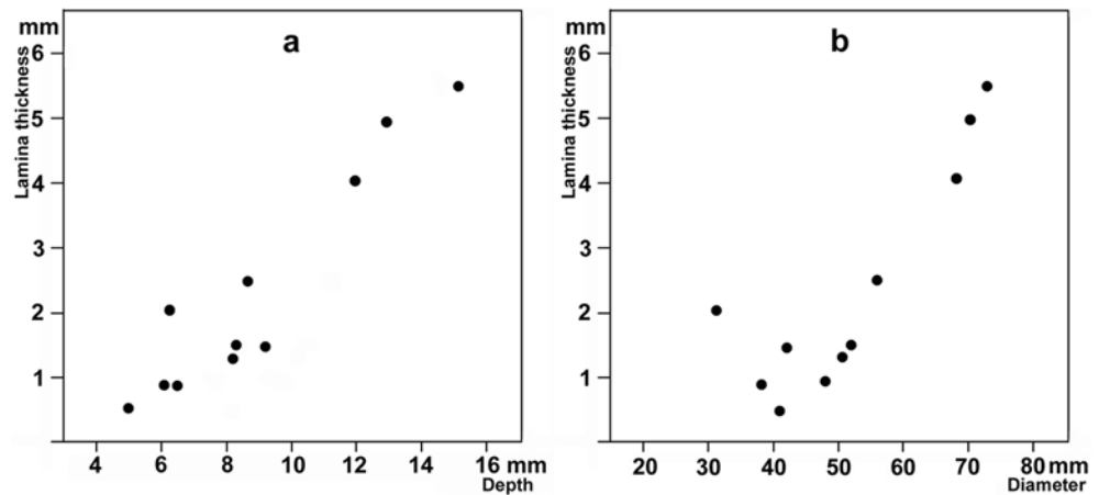
Figure 15. Metamorphosed lamina thickness plotted against (a) cupule depth and (b) cupule diameter, for a sample n = 11 cupules containing laminae formed by kinetic energy metamorphosis.
