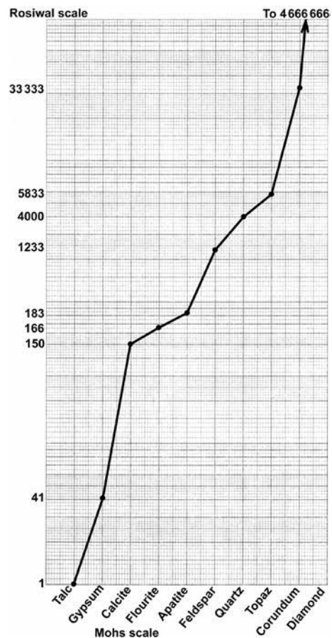
Figure 11. A comparison of Mohs scale and the Rosiwal scale, showing the irregular spacing of the former's referents and the exponential increase in abrasion resistance; note the logarithmic scale of the graph.
